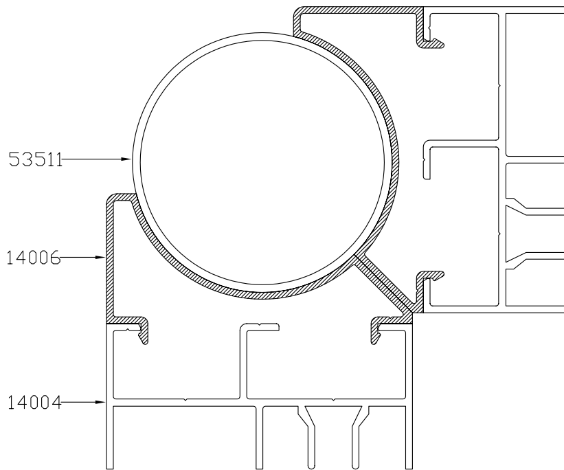
ESQUINERO REGULABLE
